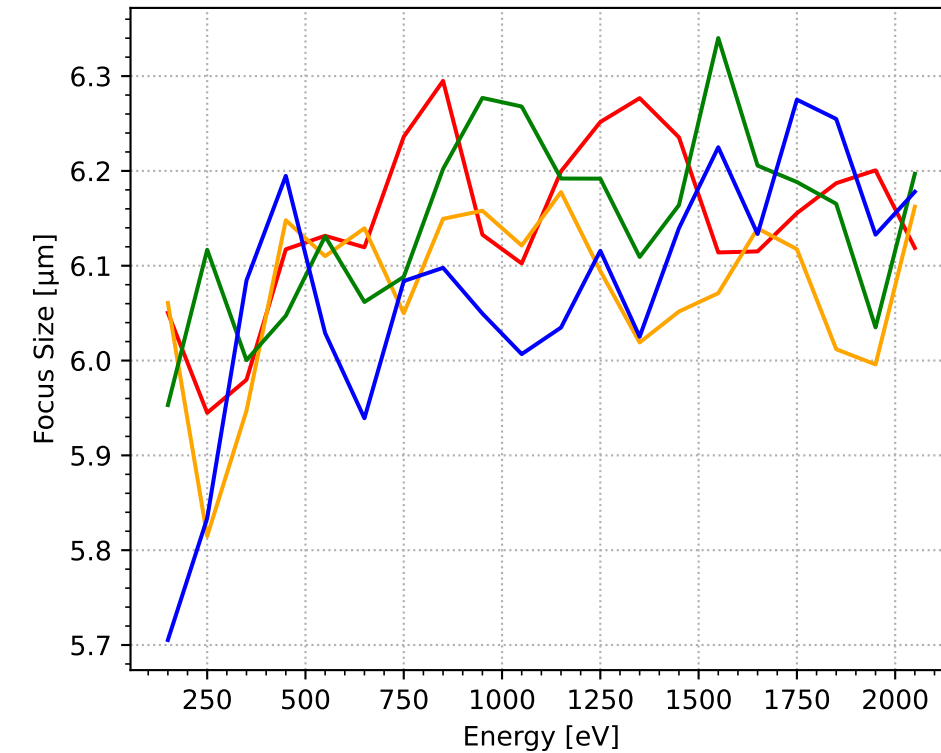
Vertical Focus
