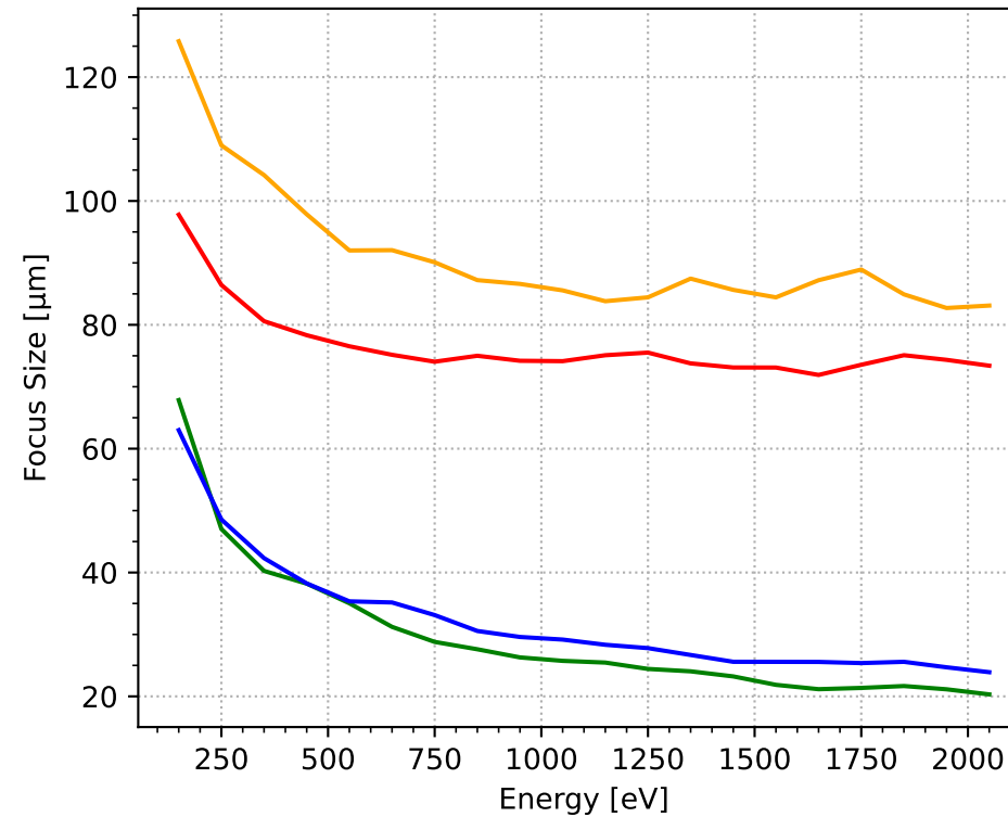
Horizontal Focus
