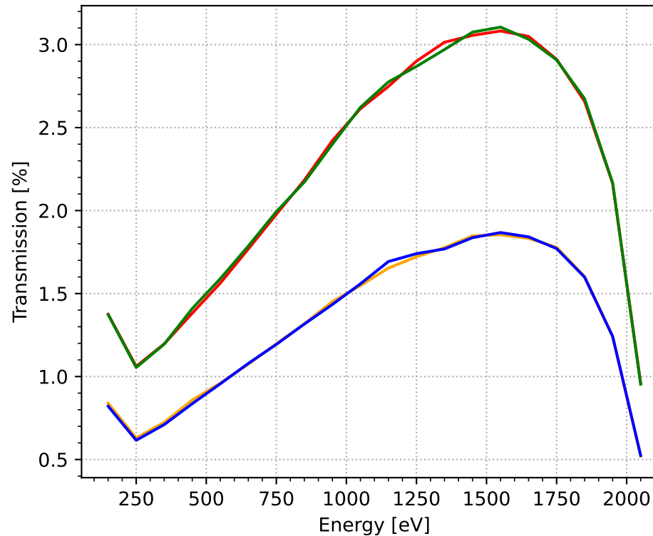
Horizontal Focus
