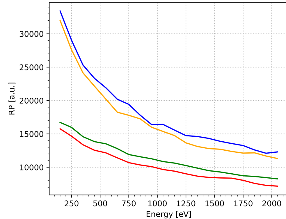
Resolving Power
